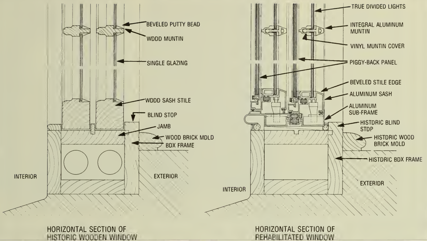
Figure 3. Horizontal section of the window shown with old and new sash. Drawing: Timothy Buehner
